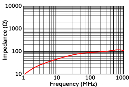
Impedance-frequency characteristics (PLT10HH450180PN)
